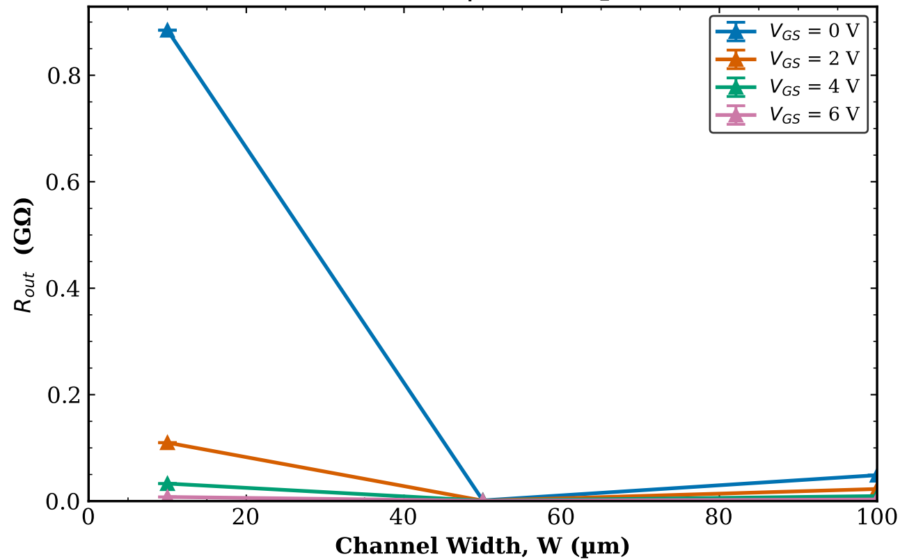
TFT3 Transistor 2 R_{out} vs W | L = 20\text{ }\mu\text{m}
